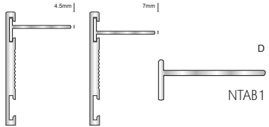
Side Profile of NSA/NTL with NTAB1
