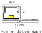
Notch to make leg removable
